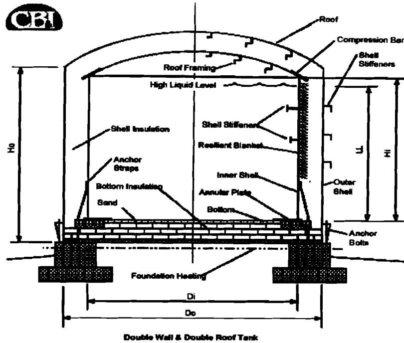
Figure 5.1: Double wall containment cryogenic vessel, CBI standard design
