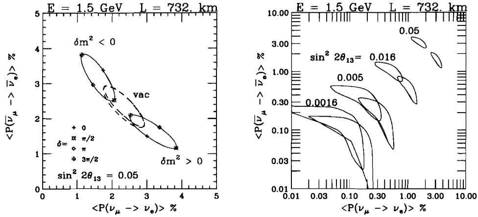
Figure 1.1: The bi-probability plots P(\nu_\mu \rightarrow \nu_e) versus P(\bar{\nu}_\mu \rightarrow \bar{\nu}_e) assuming a constant matter density of \rho = 3.0 \text{ gcm}^{-3} for an L/E of 500 km/GeV. The mixing parameters are fixed to be |\Delta m_{31}^2| = 3 \times 10^{-3} \text{ eV}^2 , \sin^2 2\theta_{23} = 1.0 , \Delta m_{21}^2 = +5 \times 10^{-5} \text{ eV}^2 , \sin^2 2\theta_{12} = 0.8 with the labeled values of \sin^2 2\theta_{13} and \delta .
