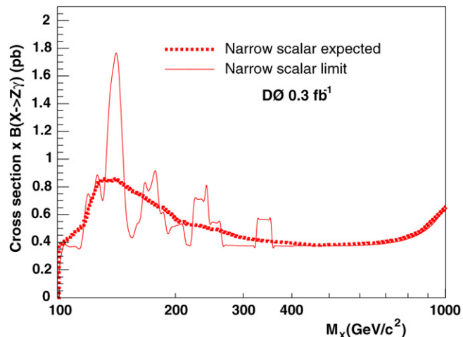
Fig. 4. The expected and observed cross section times branching fraction 95% C.L. limit for a scalar X decaying into Z\gamma as a function of M for narrow scalar.
