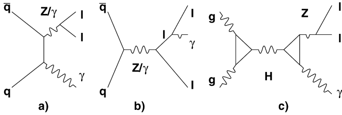
Fig. 1. The Feynman diagrams for standard model sources of di-lepton plus \gamma events are shown. Diagram (a) shows q\bar{q} \rightarrow Z -boson plus \gamma , where the photon is radiated from the quark or anti-quark. Diagram (b) shows q\bar{q} \rightarrow Z/\gamma , where the photon is radiated from one of the Z boson's decay products. Diagram (c) shows Higgs production and decay into a Z boson and a photon.
