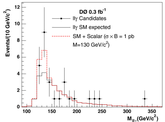
Fig. 3. Distribution of the three-body mass, M_{ll\gamma} , for candidate events and SM expectations. The signal shape for a 130 \text{GeV}/c^2 scalar decaying to Z\gamma with a \sigma(p\bar{p} \rightarrow X) \times B(X \rightarrow Z\gamma) = 1 pb is also shown.
