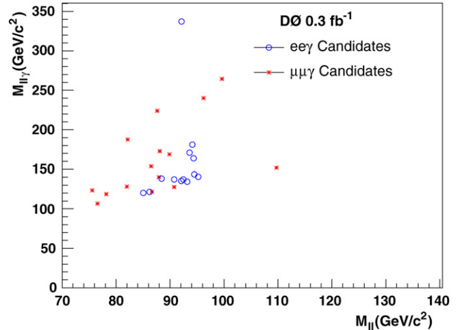
Fig. 2. Distribution of candidates in the three-body mass, M_{ll\gamma} , vs two-body mass, M_{ll} , plane is shown. The electron candidates are blue circles and the muons are red stars. The muon candidates are shown before the two-body mass constraint is applied.
