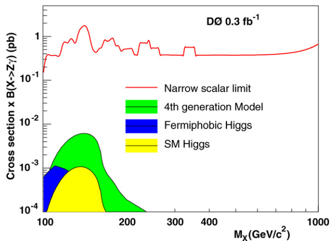
Fig. 6. The cross section times branching fraction 95% C.L. limits for a narrow scalar X decaying into Z\gamma as a function of M . Curves representing the cross section times branching ratio expected from three variations of the Higgs are shown.
