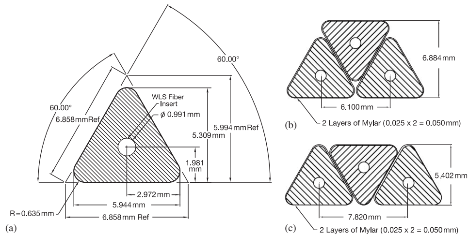
Fig. 26. Cross-section and layout geometry of the CPS and FPS scintillator strips. The circles show the location of the embedded wavelength-shifting fibers. Design dimensions are shown: (a) CPS-FPS scintillator geometry; (b) CPS geometry and (c) FPS geometry.
