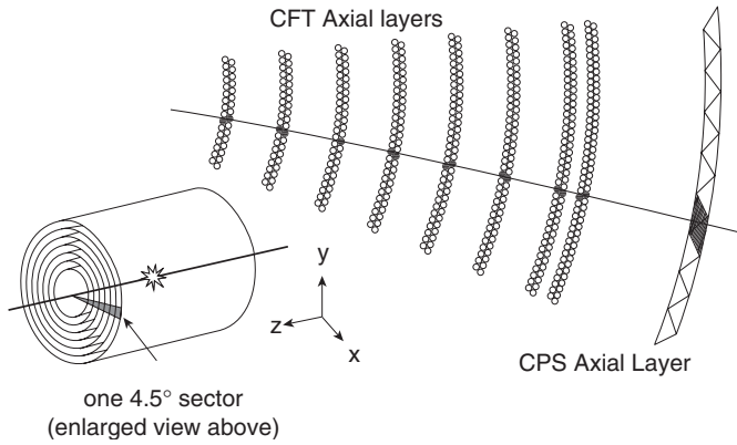
Fig. 63. Transverse schematic view of a single 4.5° sector. A hypothetical track is overlaid on the eight CFT axial doublet layers and CPS axial layer. The track equations require a fiber hit on all eight CFT axial layers. Note that the CPS is relatively farther from the CFT than shown.
