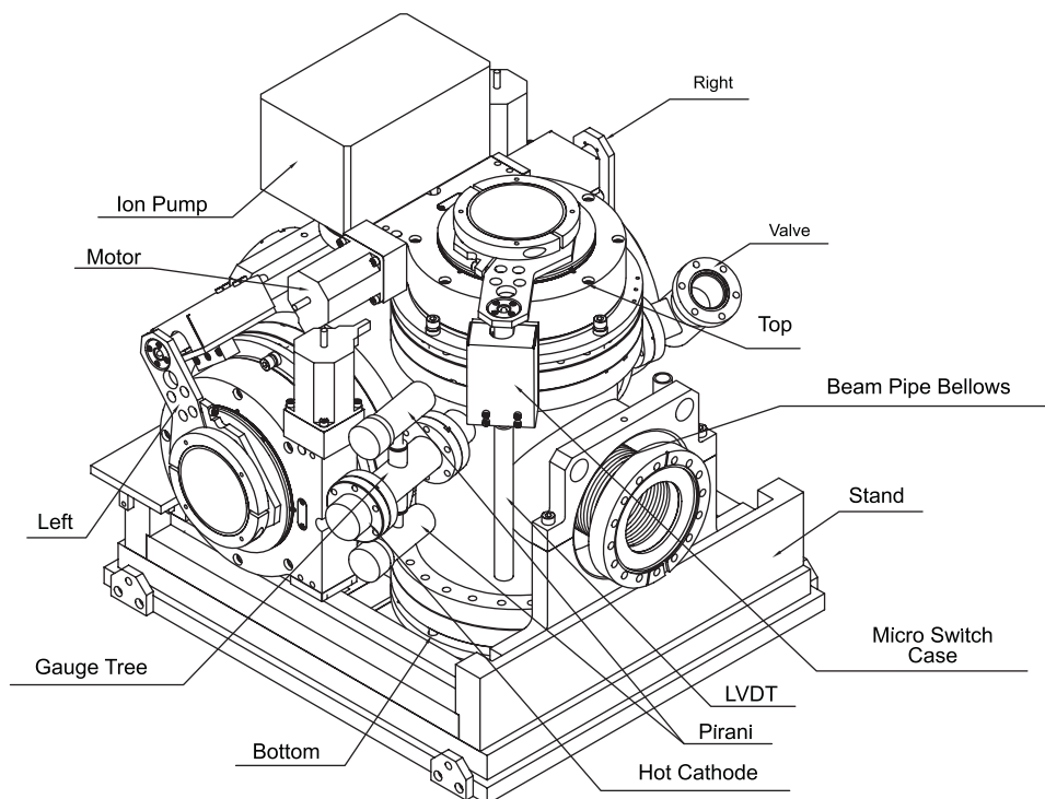
Fig. 56. FPD quadrupole castle.
