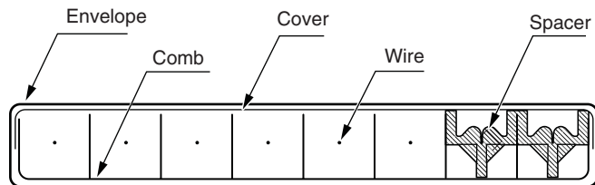
Fig. 47. Cross-sectional view of a mini drift tube.
