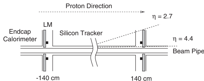
Fig. 57. Schematic drawing showing the location of the LM detectors.
