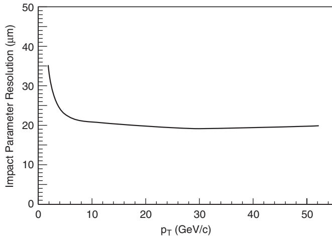
Fig. 73. Impact parameter resolution in the x, y plane as a function of p_T for simulated single muon events.
