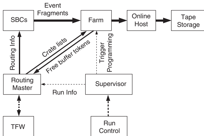
Fig. 76. Schematic illustration of the information and data flow through the L3DAQ system.
