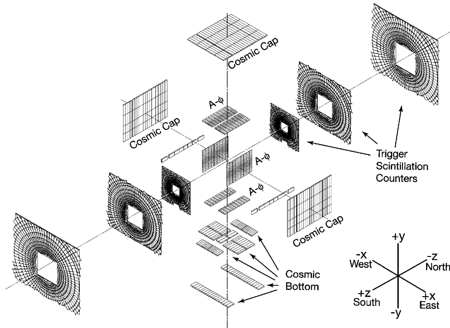
Fig. 45. Exploded view of the muon scintillation detectors.
