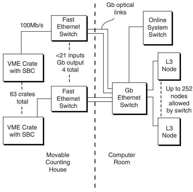
Fig. 75. The physical network configuration of the L3DAQ system. The moveable counting house holds electronics for the detector and moves with the detector between the assembly hall and the collision hall.
