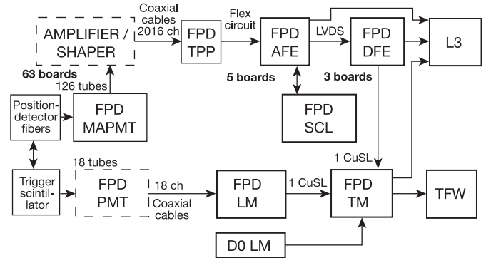
Fig. 67. A schematic view of the L1FPD trigger. The dashed boxes indicate Run I surplus boards; the bold boxes indicate Run II standard; and the thin boxes indicate custom FPD electronics. CuSL is a copper serial link.
