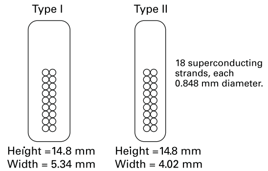
Fig. 22. Cross-sections of the two conductors used in construction of the solenoidal magnet.
