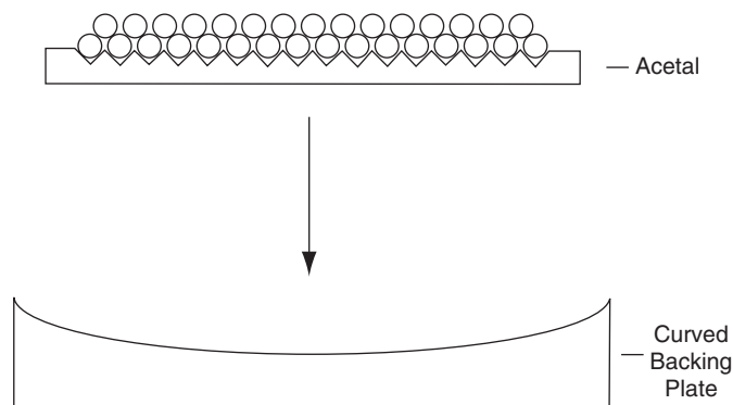
Fig. 13. Technique for curved scintillating fiber ribbon fabrication.
