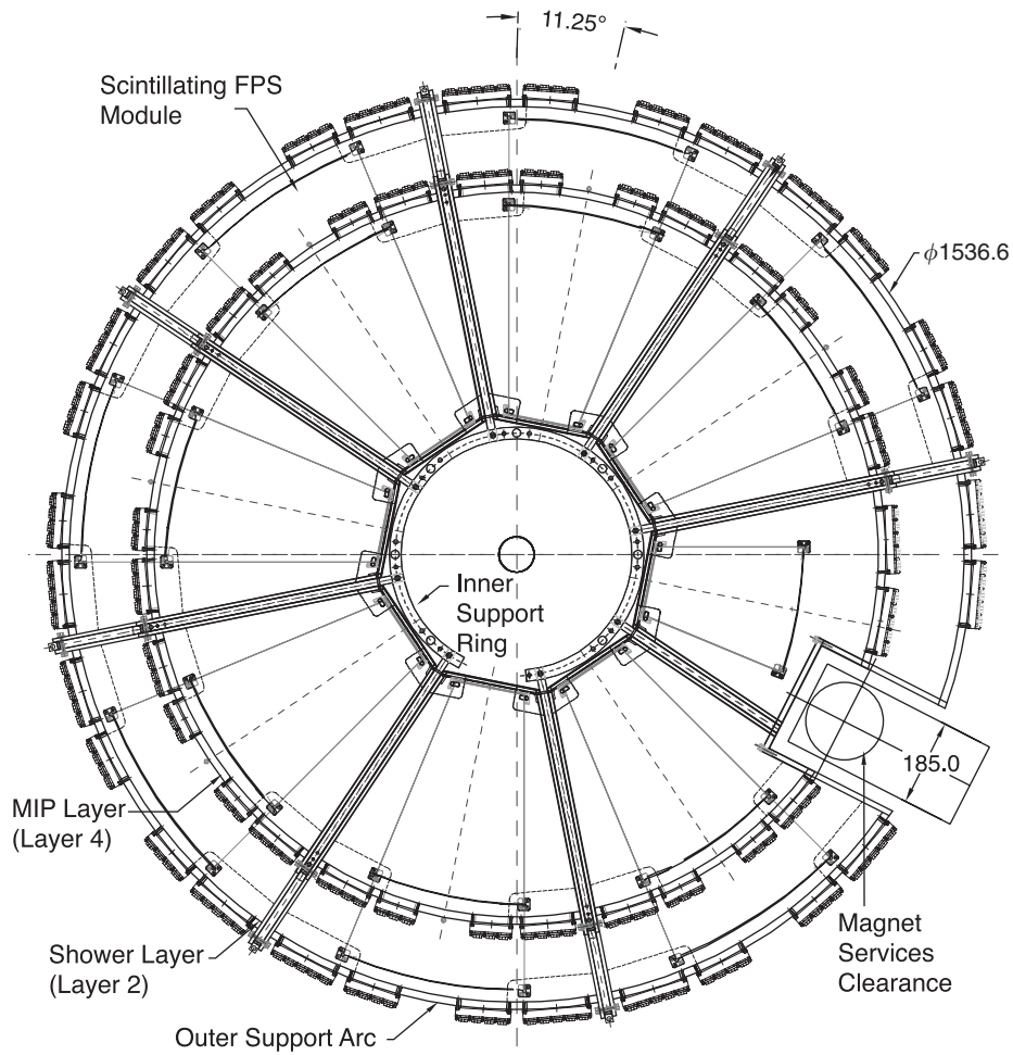
Fig. 30. r-\phi view of the north FPS detector. For clarity, only layers 2 (shower) and 4 (MIP) are shown; layers 1 (shower) and 3 (MIP) are rotated by 22.5^\circ in \phi with respect to these layers so their supports do not overlap. The south FPS detector is a mirror image of the north detector. The cutback near four o'clock accommodates the solenoidal magnet cryogenic services on the south side.
