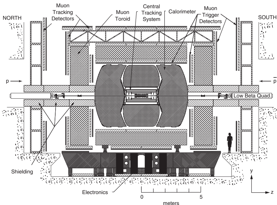
Fig. 1. Diagram of the upgraded D\bar{O} detector, as installed in the collision hall and viewed from inside the Tevatron ring. The forward proton detector is not shown. The detectors in the central region of the detector are shown in Fig. 2.
