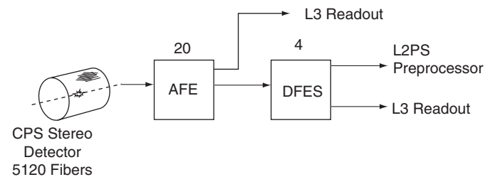
Fig. 64. CPS stereo subsystem hardware.
