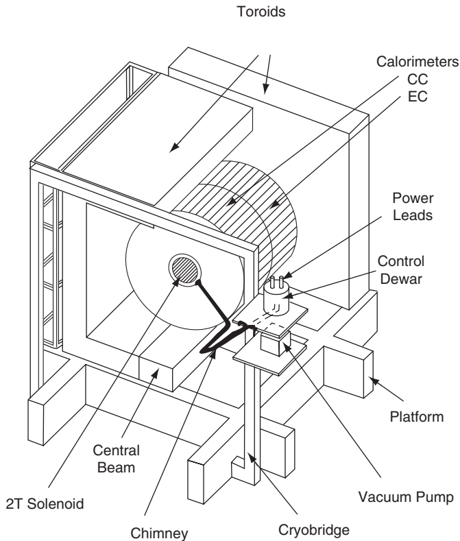
Fig. 21. Perspective view of the solenoid inside the central calorimeter. One end calorimeter, several muon chambers, and parts of the toroids have been omitted for clarity. Also shown are the service chimney and control dewar.
