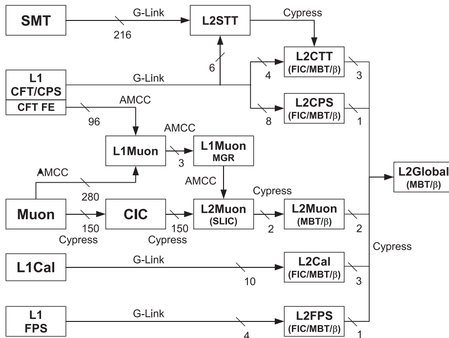
Fig. 68. L2 data paths and connections. Data paths are labeled according to transmission protocol, either 1.3Gb/s fiber G-Links, 160Mb/s copper Cypress Hotlinks, or 1.4Gb/s copper AMCC links. FIC indicates a fiber converter card, MBT an Mbus transceiver card, and \beta an L2 \beta card. The number of transmission cables is given for each pathway.
