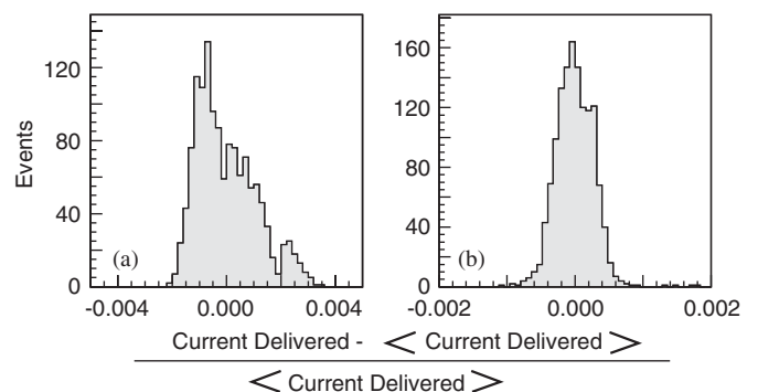
Fig. 38. The mean current/DAC delivered by the pulser boards is 0.825\ \text{mA}/\text{DAC} with a spread of (a) 0.2% for all 15 pulser boards produced and (b) 0.1% within one board.
