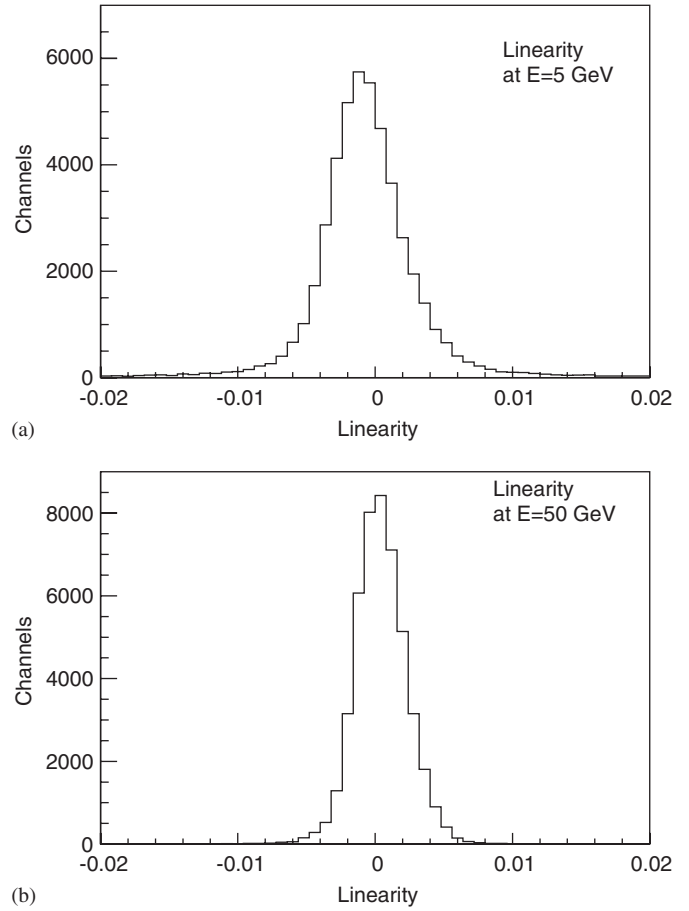
Fig. 40. Linearity defined as \text{ADC}_{\text{measured}}/\text{ADC}_{\text{fit}} - 1 and determined from pulser calibration data at (a) 5 GeV and (b) 50 GeV.
