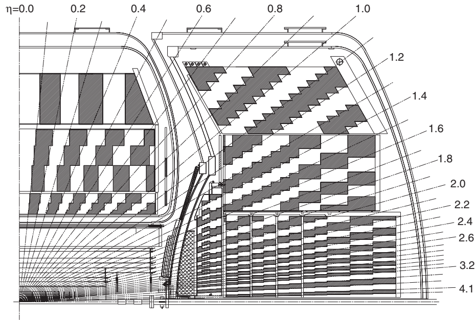
Fig. 34. Schematic view of a portion of the D0 calorimeters showing the transverse and longitudinal segmentation pattern. The shading pattern indicates groups of cells ganged together for signal readout. The rays indicate pseudorapidity intervals from the center of the detector.
