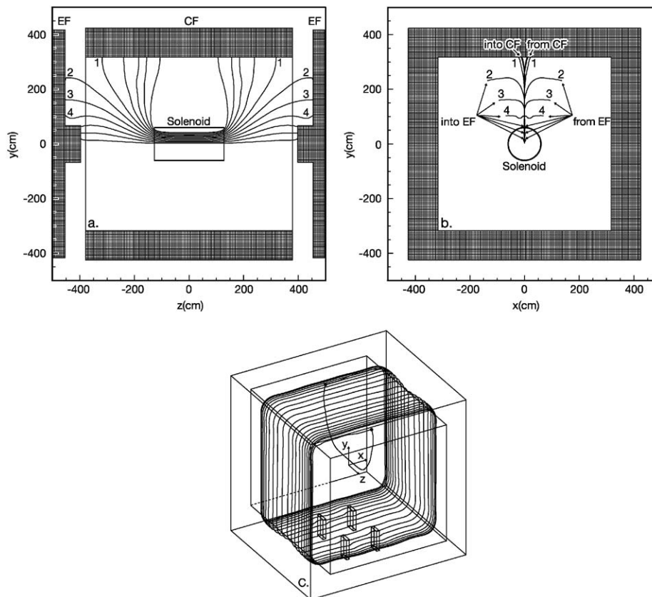
Fig. 25. Details of the magnetic field; CF is the central toroid and the EFs are the end toroids. (a) Some of the y - z projection field lines that are shown in Fig. 24. (b) The same lines in the y - x projection. The lines appear to stop short because they end at the x position at which they enter the toroid. (c) A complete view of one of the field lines; it enters the central toroid at x, z < 0 , wraps around the toroid, and exits at x, z > 0 .
