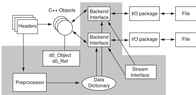
Fig. 81. The structure of DØOM. The shaded area shows the components which are part of DØOM proper.
