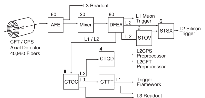
Fig. 62. The CFT/CPS axial components of the L1CTT system. The numbers in the top left corners of the boxes indicate the number of board of each type.
