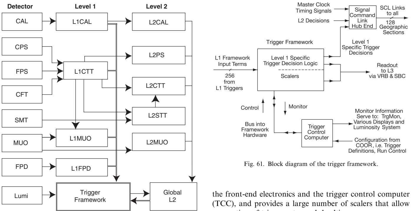
Fig. 60. Block diagram of the DØ L1 and L2 trigger systems. The arrows show the flow of trigger-related data.
