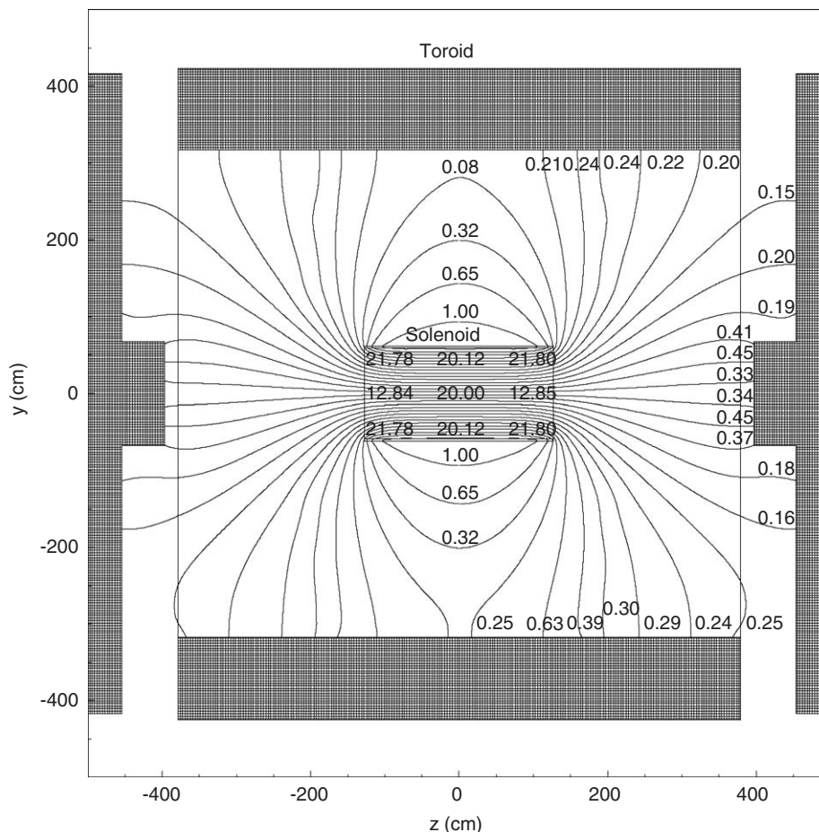
Fig. 24. A y - z view of the DØ magnetic field (in kG) with both the toroidal and solenoidal magnets at full current (1500 and 4749 A, respectively). The field in the central toroid is approximately 1.8 T; that in the end toroids is about 1.9 T. The field lines are projections onto the y - z plane; all lines start at x = 0 when z = 0 but the left and right line ends differ by up to 2.5 m in x (see Fig. 25 for more details).
