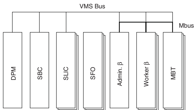
Fig. 70. Layout of cards in an L2Muon crate. Two stages of processing are completed in a single crate using SLICs and L2 \beta processors. Central and forward muon regions are processed in separate crates of similar configuration.
