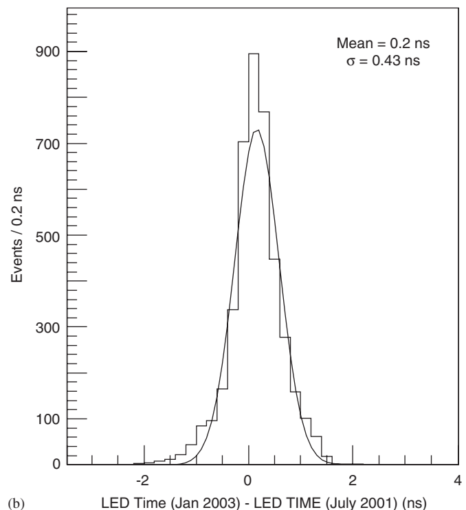
Fig. 52. Results from the forward muon system monitoring by the LED calibration system over one and one-half years; the smooth curves are Gaussian fits to the data. (a) Shows the LED amplitude ratio, (b) shows the absolute difference in the LED timing.
