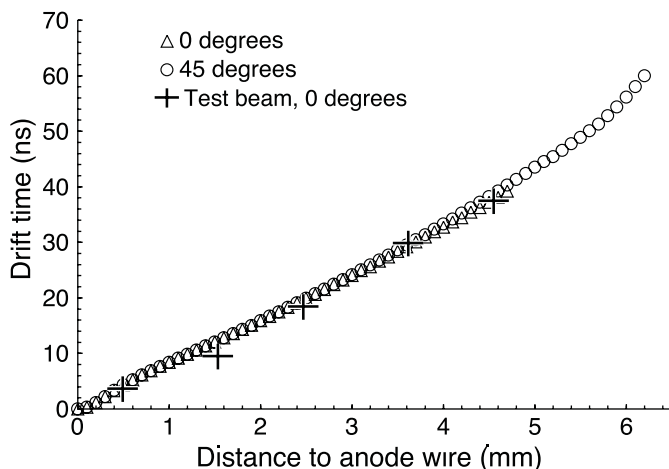
Fig. 48. Time-to-distance relationship for a mini drift tube. The points labeled 0^\circ and 45^\circ are calculated using GARFIELD. The crosses indicate measurements done at 0^\circ .
