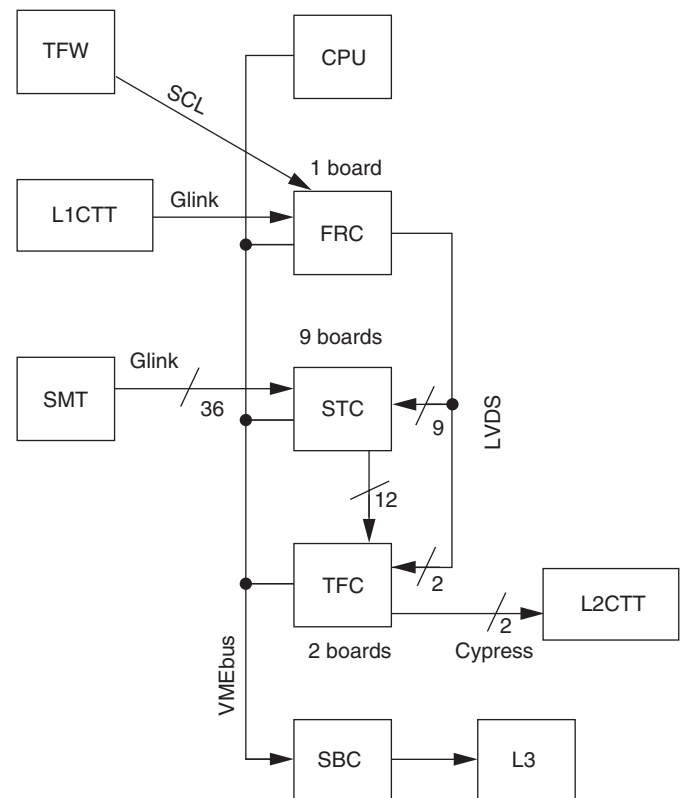
Fig. 72. Data flow through an L2STT crate.
