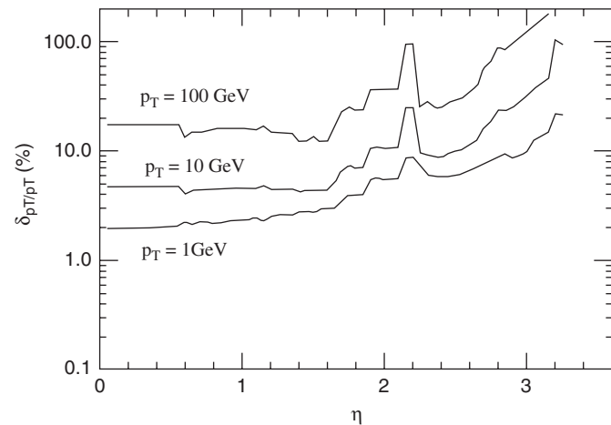
Fig. 3. Expected relative transverse momentum resolution of the central tracking system as a function of pseudorapidity for tracks with p_T = 1, 10, and 100 \text{ GeV}/c .
