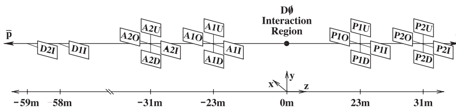
Fig. 54. FPD layout. Quadrupole castles are designated with a leading P or A when placed on the p side or the \bar{p} side, respectively; the number designates the station location; while the final letter indicates pot position (U for up, D down, I in, O out). D1I and D2I are dipole castles.
