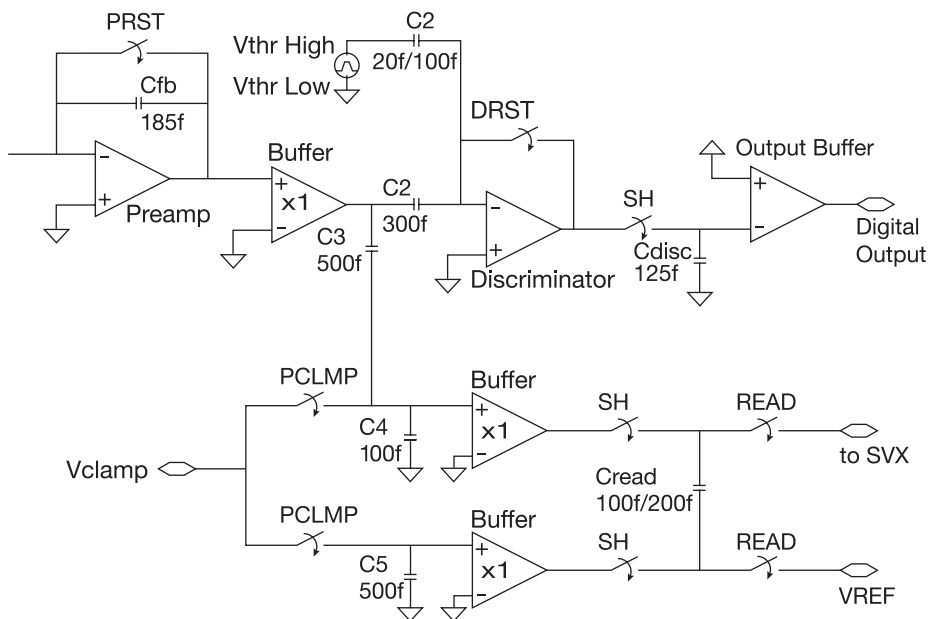
Fig. 19. Simplified schematic diagram of the SIFT chip. Vclamp, Vthr, and VREF are externally supplied DC voltage levels.
