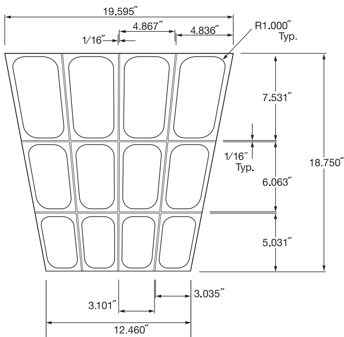
Fig. 43. Each ICD tile is subdivided into 12 straight-edged trapezoidal subtiles. WLS fibers for readout are embedded into each subtile along the curved trapezoids.
