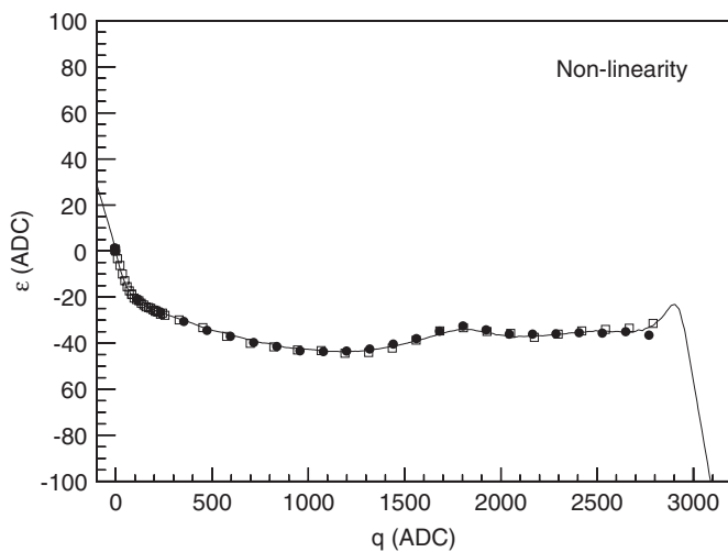
Fig. 39. The SCA non-linearity \varepsilon as a function of the equivalent preamplifier input charge q compared to the residuals u - a \cdot S + \varepsilon(p) of pulser calibration data for a given channel. The data for the \times 8 gain path ( \times 1 gain path divided by 8) are shown by the open squares (solid circles). Uncertainties corresponding to the dispersion \sigma/\sqrt{N} of the measured ADC values for the 100 events taken at each pulse height are smaller than the symbols.
