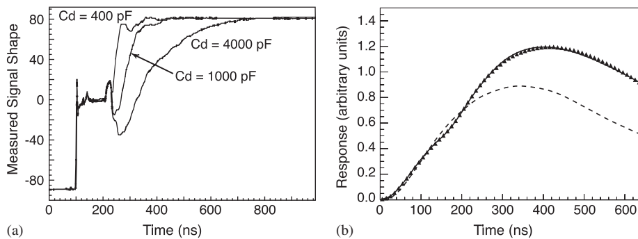
Fig. 41. Reflection measurements used to determine the cable resistivity, the cell capacitance (Cd), and the feedthrough and signal strip inductance. (a) The measured response function for three different channels to a step function as a function of time. The vertical voltage scale is in arbitrary units. These parameters are used in a simulation model to study the response function to a calibration signal and a physics signal. (b) The measured response function of a calibration signal for an electromagnetic channel (triangles) is compared to the response obtained from the simulation (solid line) and the predicted response to a physics signal (dashed line).
