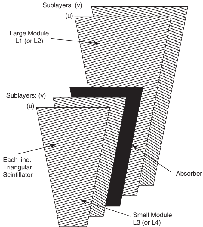
Fig. 28. Complete \phi -segment of a FPS module showing the overlapping u-v MIP and shower layers, separated by a lead and stainless steel absorber.
