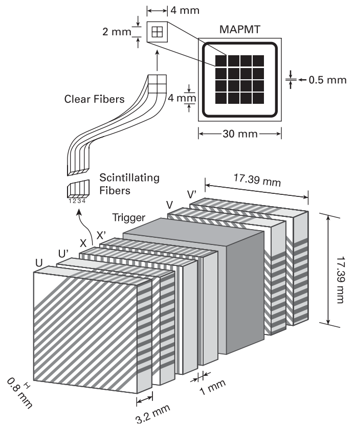
Fig. 55. Detector fibers and the MAPMT.
