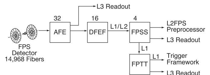
Fig. 65. FPS subsystem hardware.
