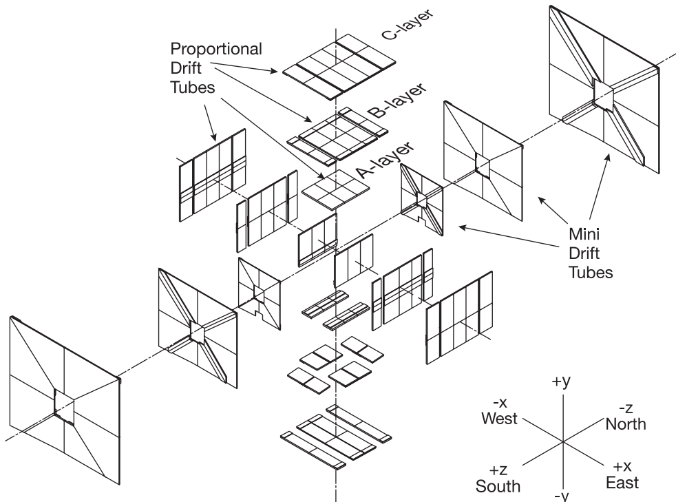
Fig. 44. Exploded view of the muon wire chambers.
