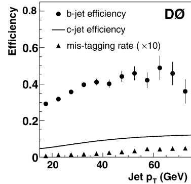
Fig. 1. Measured b -tagging efficiency (circles) and mistagging rate (triangles), and estimated c -tagging efficiency (solid line) as a function of jet p_T .
