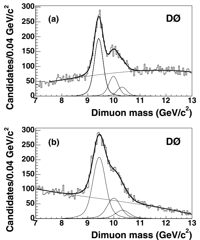
FIG. 1. Example of fits to the dimuon spectra in different bins of rapidity in the p_T bin of 4 < p_T^Y < 6 GeV/ c : (a) |y^Y| \leq 0.6 , (b) 1.2 < |y^Y| \leq 1.8 . The heavy line shows the combined fit for signal and background. Also shown are the individual contributions from the three Y states and the background separately.
