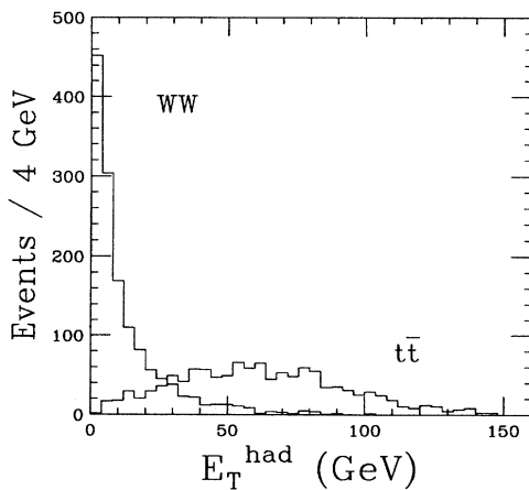
FIG. 1. E_T^{\text{had}} for Monte Carlo WW and t\bar{t} events with M_{\text{top}} = 160 \text{GeV}/c^2 ( \int L dt \sim 20 \text{fb}^{-1} ). Events with E_T^{\text{had}} \geq 40 \text{GeV} were rejected.
