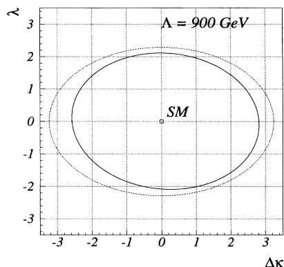
FIG. 2. 95% CL limits on the CP -conserving anomalous couplings \lambda and \Delta\kappa , assuming that \lambda_\gamma = \lambda_Z and \kappa_\gamma = \kappa_Z . The dotted contour is the unitarity limit for the form factor scale \Lambda = 900 GeV which was used to set the coupling limits.
