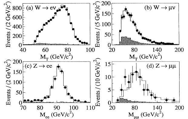
FIG. 1. Transverse mass and invariant mass distributions for the indicated channels. The points are the data. The shaded areas represent the estimated backgrounds, and the solid lines correspond to the sums of the expected signals (from Monte Carlo) and the estimated backgrounds.
