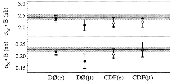
FIG. 2. \sigma B for inclusive W and Z boson production. The inner error bar is the combined statistical and systematic uncertainty and the outer error bar includes the luminosity uncertainty. The solid line and shaded band are the theoretical prediction described in the text.
