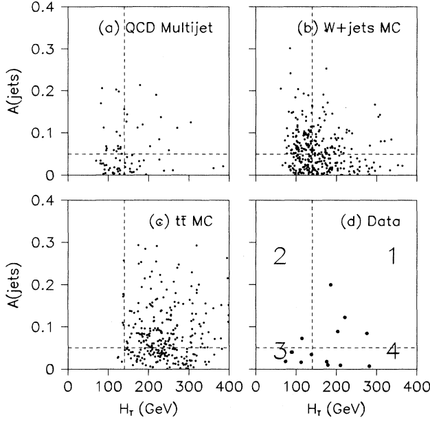
FIG. 25. \mathcal{A} vs H_T distributions for events with four or more jets: (a) QCD multijet sample, (b) VECBOS Monte Carlo program, (c) t\bar{t} events, top mass 180 \text{ GeV}/c^2 , (d) data e and \mu + jets combined; the quadrants used in the fit are numbered, see Sec. VIID.
