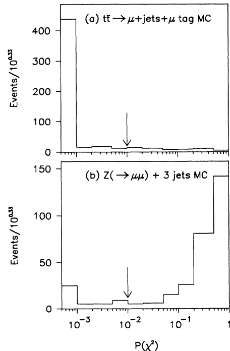
FIG. 41. The \chi^2 probability distribution for (a) simulated t\bar{t} \rightarrow \mu + \text{jets} + \mu\text{-tag} events ( m_t = 160 \text{ GeV}/c^2 ) and (b) simulated Z(\rightarrow \mu\mu) + 3 \text{ jet} events.
