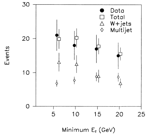
FIG. 35. Comparison of background predictions and data for electron + 1 jet + muon-tag events with \cancel{E}_T > 20 GeV as a function of the minimum jet E_T .
