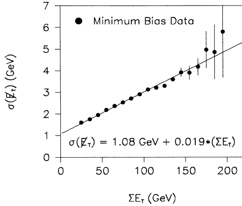
FIG. 10. Uncorrected \cancel{E}_{Tx}^{\text{cal}} distribution for minimum bias data. The line represents a fit to the data points.
