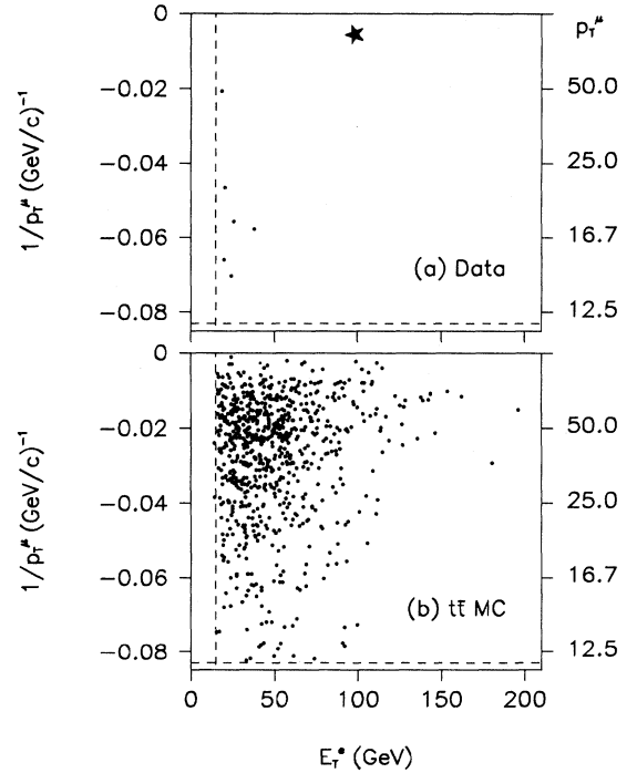
FIG. 16. 1/p_T^\mu vs E_T^e for (a) D0 data and (b) t\bar{t} \rightarrow e\mu Monte Carlo events ( m_t = 170 GeV/ c^2 , \int \mathcal{L} dt = 21 fb ^{-1} ). The dashed lines represent the selection cuts on 1/p_T^\mu and E_T^e .
