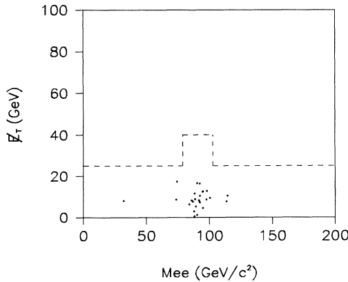
FIG. 15. E_T vs M_{ee} for D0 data. The dashed line is the cut (see text).
