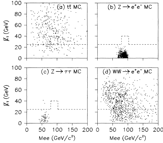
FIG. 14. E_T vs M_{ee} for (a) t\bar{t} \rightarrow ee + X ( m_t = 140 \text{ GeV}/c^2 ), (b) Z \rightarrow ee , (c) Z \rightarrow \tau\tau , and (d) WW \rightarrow e\nu e\nu Monte Carlo samples corresponding to an integrated luminosity of 12.1 \text{ pb}^{-1} , 47.7 \text{ pb}^{-1} , 0.53 \text{ fb}^{-1} , 21.2 \text{ fb}^{-1} , respectively. Dashed line represents the cut (see text).
