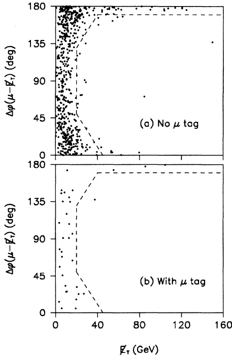
FIG. 39. The correlation of the angle \Delta\phi between the total \cancel{E}_T and the highest p_T muon with the total \cancel{E}_T for multijet events having a nonisolated high- p_T muon (a) without and (b) with an additional tagging muon.
