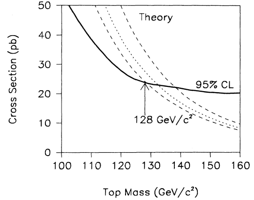
FIG. 44. 95% confidence level on \sigma_{t\bar{t}} as function of top mass from low mass analysis. Also shown are central (dotted line), high, and low (dashed lines) theoretical cross section curves [21].
