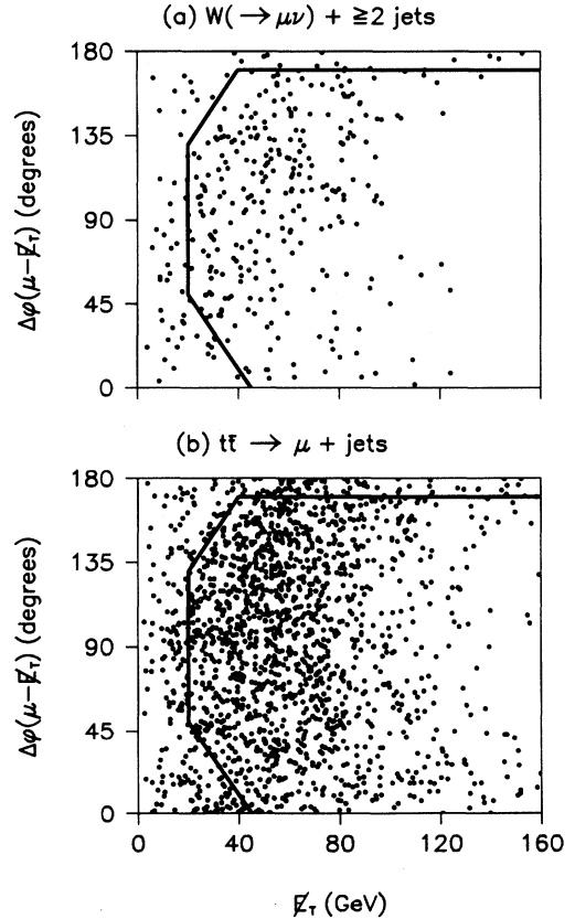
FIG. 40. The correlation of the angle \Delta\phi between the total \cancel{E}_T and the highest p_T muon with the total \cancel{E}_T for simulated W + \text{jets} and t\bar{t} events ( m_t = 160 \text{ GeV}/c^2 ). The luminosities of the two samples are 80 \text{ pb}^{-1} and 3240 \text{ pb}^{-1} , respectively.
