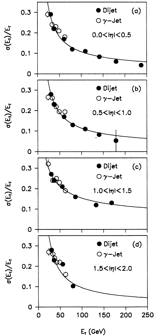
FIG. 8. Jet energy resolution as a function of the average corrected jet E_T as computed from dijet events and photon jet events in four pseudorapidity regions. Fits to the resolution function in these \eta regions are also shown.
