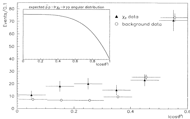
FIG. 3. Center of mass angular distribution of \gamma\gamma candidates.
