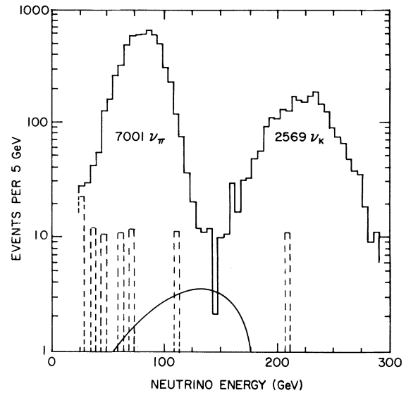
FIG. 1. Solid histogram: Distribution in observed total energy for events inside a single radial bin of interaction points at the target ( 25.4 \text{ cm} < R < 50.8 \text{ cm} ) for the + 250 GeV/c fast-spill data. This separation is typical of data at all radii and beam settings. (Note the logarithmic scale.) Dashed histogram: Observed energy distribution for events obtained when the entrance to the decay region is blocked (wide-band background). These data have been normalized to the same number of incident protons as the data in the solid curve. Smooth curve: Calculated \nu_\mu events from K_{\mu 3} -decay neutrinos, normalized to the events in the \nu_K peak.
