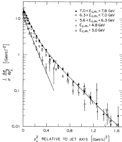
FIG. 25. Corrected (1/\sigma)d\sigma/dp_{\perp}^2 vs p_{\perp}^2 for particles opposite (negative x_{||} ) jets with x_{\max} > 0.3 for various E_{\text{c.m.}} . p_{\perp} is the component of particle momentum perpendicular to the jet direction. The distributions are normalized to the cross sections for jets with x_{\max} > 0.3 . The solid lines represent the fits, discussed in the text, to the distributions for E_{\text{c.m.}} = 3.0 GeV and 7.0 < E_{\text{c.m.}} < 7.8 GeV.
