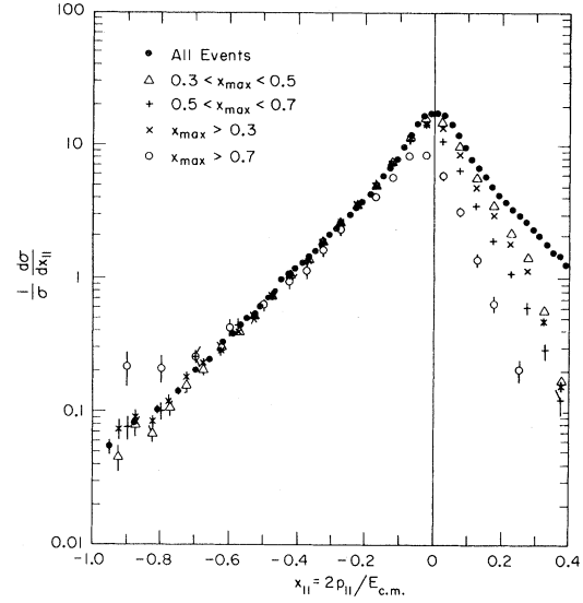
FIG. 18. Corrected particle-density distributions (1/\sigma)d\sigma/dx_{||} vs x_{||} for various x_{\text{max}} cuts for 7.0 < E_{\text{c.m.}} < 7.8 GeV. x_{\text{max}} is the highest- x particle on one side of the event and is not plotted. The jet direction is oriented so that x_{\text{max}} is at positive x_{||} . The distributions are normalized to the cross sections for jets with x_{\text{max}} within the specified range.
