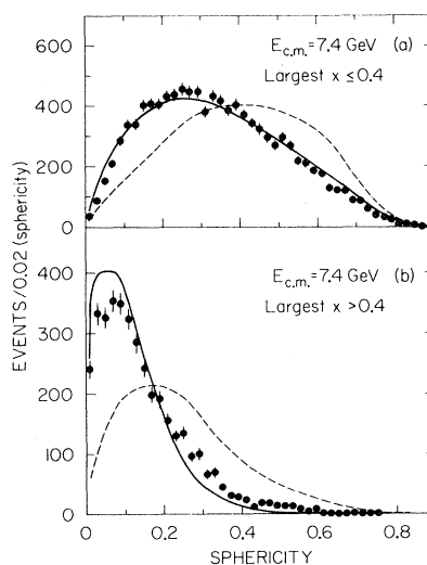
FIG. 8. Observed sphericity distributions at 7.4 GeV for data, jet model (solid curves), and phase-space model (dashed curves) for (a) events with largest x \leq 0.4 and (b) events with largest x > 0.4 .
