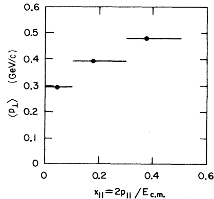
FIG. 34. Average transverse momentum relative to the jet direction \langle p_{\perp} \rangle vs x_{\parallel} for particles opposite jets with x_{\max} > 0.3 for 7.0 < E_{\text{c.m.}} < 7.8 GeV.
