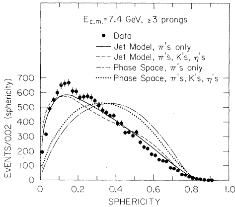
FIG. 4. Observed sphericity distribution at 7.4 GeV compared with prediction for jet model with pions only (solid curve), jet model with pions, kaons, and \eta 's (dashed curve), phase-space model with pions only (dashed-dotted curve), and phase-space model with pions, kaons, and \eta 's (dotted curve).
