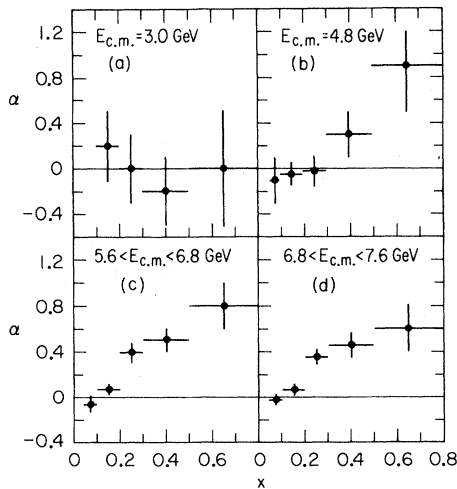
FIG. 14. Inclusive hadron angular distribution coefficient \alpha vs x obtained from fits to 1 + \alpha(x)\cos^2\theta for (a) E_{c.m.} = 3.0 GeV, (b) E_{c.m.} = 4.8 GeV, (c) 5.6 < E_{c.m.} < 6.8 GeV, and (d) 6.8 < E_{c.m.} < 7.6 GeV.
