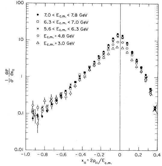
FIG. 20. Corrected particle-density distributions (1/\sigma)d\sigma/dx_{||} vs x_{||} for x_{\max} > 0.3 for various E_{c.m.} . x_{\max} is at positive x_{||} and is not plotted. The distributions are normalized to the cross sections for jets with x_{\max} > 0.3 .
