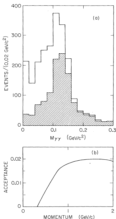
FIG. 1. (a) \gamma\text{-}\gamma invariant-mass distribution for events with two or more \gamma 's detected in the LGW. A \gamma -energy cutoff of 150 MeV is required for events in the shaded region. (b) \pi^0 acceptance in the LGW as a function of \pi^0 momentum for isotropically produced \pi^0 's.
