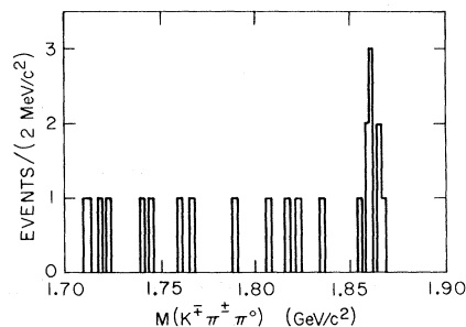
FIG. 3. K^+\pi^+\pi^0 invariant-mass distribution for constrained events with a \chi^2 = 5 cutoff.
