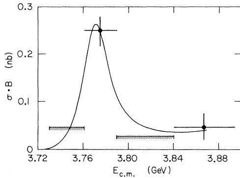
FIG. 1. \sigma B for D^0 (\bar{D}^0) \rightarrow K^\mp \pi^\pm as a function of E_{c.m.} . The cross-hatched bars represent 90%-confidence-level upper limits. The curve represents the fit to the \psi'' line shape and charmed-particle background from Ref. 1 normalized to the E_{c.m.} = 3.774 GeV point.
