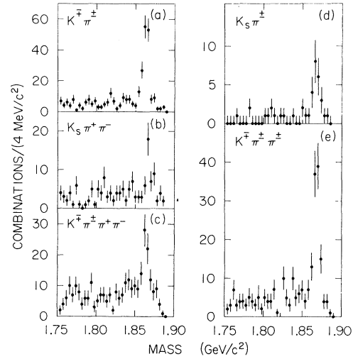
FIG. 2. Invariant-mass spectra for various D decay modes. See text for a discussion of cuts and techniques.
