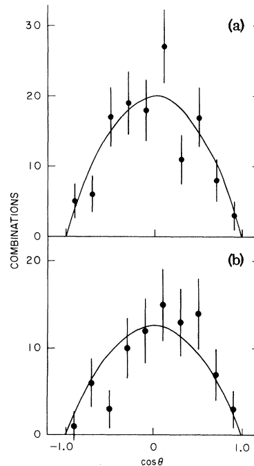
FIG. 3. Cosine of the angle between the incident e^+ beam and the D momentum for (a) D^0 ( \bar{D}^0 ) \rightarrow K^{\mp}\pi^{\pm} and (b) D^+ \rightarrow K^{\mp}\pi^{\pm}\pi^{\pm} , after background subtraction. The curves represent \sin^2\theta , the required distribution for the production of spinless D mesons.
