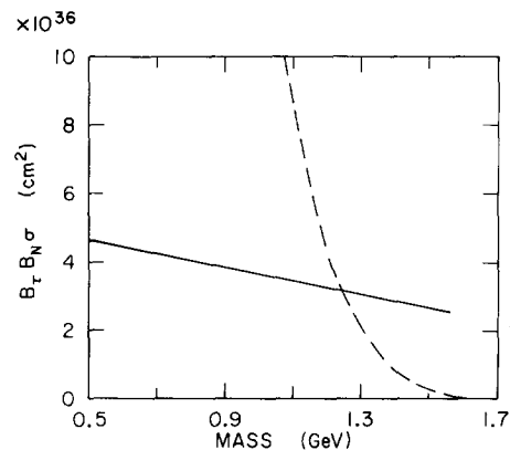
Fig. 2. The solid curve gives the 90% confidence upper limit for an l\pi mass peak. The dashed curve is the theoretical estimate based on expected \tau and N branching ratios and \tau pair production of one unit of R .
