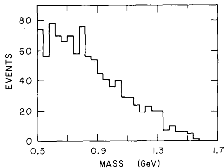
Fig. 1. Number of events detected as a function of l\pi mass.
