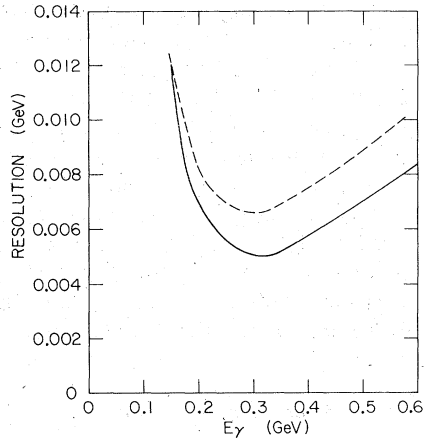
FIG. 4. Photon rms energy resolution versus photon energy. The solid line indicates the effect of the momentum resolution of charged particles. The dashed line includes also the effect of energy loss by ionization and radiation.
