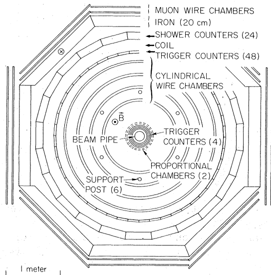
FIG. 1. An end view of the magnetic detector. The iron flux return and muon chambers were removed from the two side sections for much of the running.
