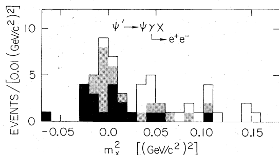
FIG. 7. The missing mass squared recoiling against \psi\gamma in \psi\gamma\gamma candidates with one photon converted. The shading is discussed in the text.
