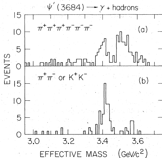
FIG. 11. Mass spectrum for multihadron state X fit to the reaction \psi' \rightarrow \gamma X with X being (a) \pi^+\pi^-\pi^+\pi^-\pi^+\pi^- , (b) \pi^+\pi^- or K^+K^- .
