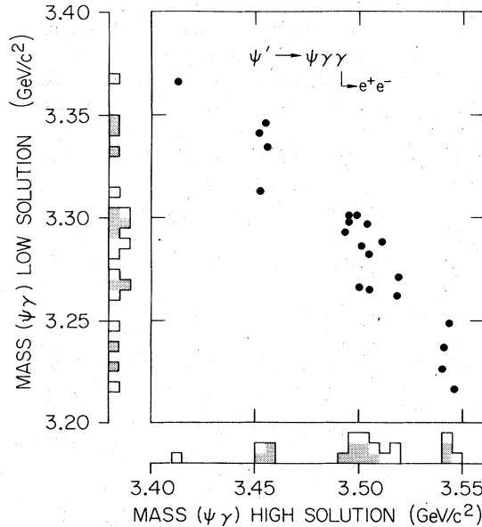
FIG. 9. The two solutions for \psi\gamma masses from 21 \psi\gamma\gamma events.
