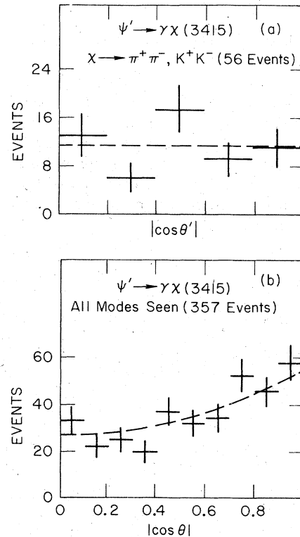
FIG. 13. Decay angular distributions for \chi(3415) . Angles are defined in text and dashed lines represent the predictions for J=0 .
