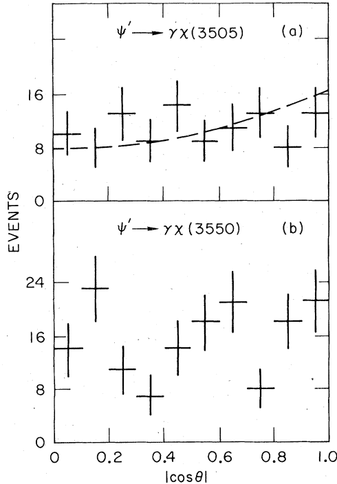
FIG. 14. Angular distributions for (a) \chi(3505) and (b) \chi(3550) . The dashed line represents the predictions for J=0 .
