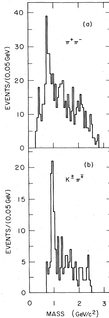
FIG. 12. (a) \pi^+\pi^- mass spectrum from \chi(3415) \rightarrow \pi^+\pi^-\pi^+\pi^- (four combinations per event); (b) K^+\pi^- mass spectrum from \chi(3415) \rightarrow \pi^+\pi^-K^+K^- (two combinations per event).
