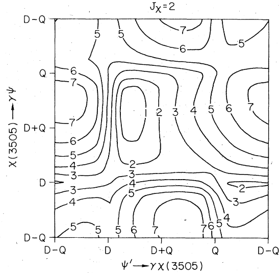
FIG. 18. Likelihood function assuming J_\chi = 2 as a function of the relative dipole and quadrupole amplitudes for each decay, assuming the octupole amplitudes are zero. The contours are explained in the text. The scale is the same as that for the preceding figure.
