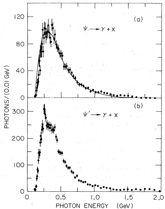
FIG. 5. (a) The inclusive photon spectrum from \psi . The solid line is the spectrum from a Monte Carlo simulation of \psi events. (b) The inclusive photon spectrum from \psi' .
