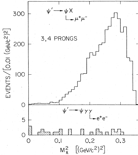
FIG. 8. Missing mass squared recoiling against the \psi for the 27 \psi\gamma\gamma events and also for all 3- and 4-prong events in which a \psi was detected.
