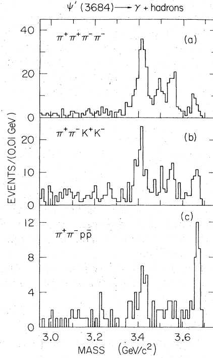
FIG. 10. Mass spectrum for multihadron state X fit to the reaction \psi' \rightarrow \gamma X with X being (a) \pi^+\pi^-\pi^+\pi^- , (b) \pi^+\pi^-K^+K^- , (c) \pi^+\pi^-p\bar{p} .
