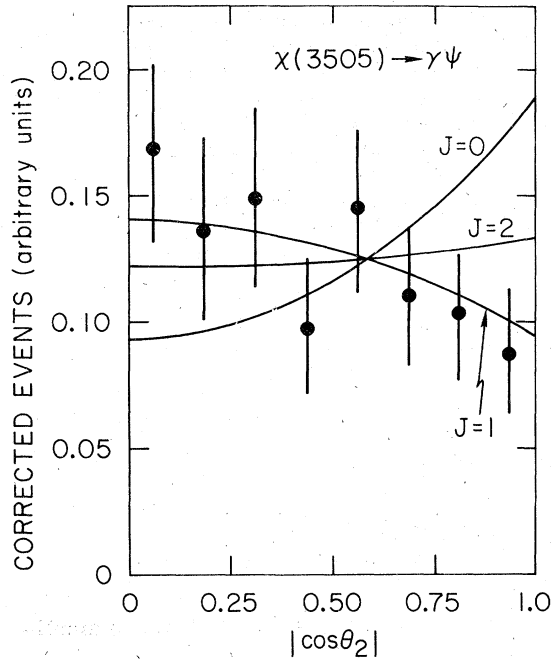
FIG. 16. Cosine of the angle between the photon direction and the lepton direction in \chi \rightarrow \gamma\psi ; \psi \rightarrow l^+l^- . The data have been corrected for acceptance biases. The solid curves represent predicted curves for a given \chi spin, assuming pure dipole decay.
