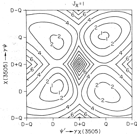
FIG. 17. Likelihood function assuming J_\chi = 1 as a function of the relative dipole and quadrupole amplitudes for each decay. The contours are explained in the text. D indicates pure dipole decay, and Q pure quadrupole decay. D \pm Q indicate equal dipole and quadrupole amplitudes with the relative phase indicated. The scale is linear in the square of either amplitude.
