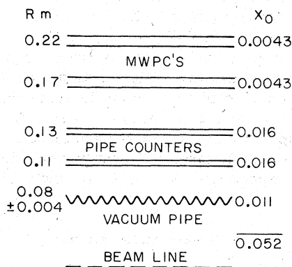
FIG. 2. The effective converter, with thickness and distance from the beam line.
