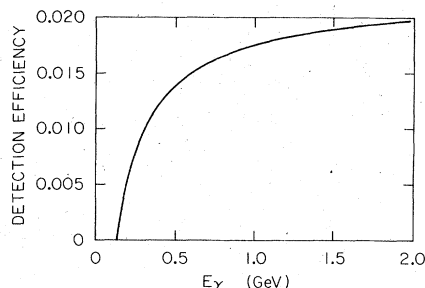
FIG. 3. Photon-detection efficiency versus photon energy.
