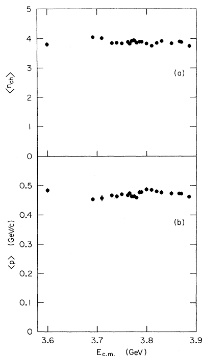
FIG. 1. (a) Observed mean charged-particle multiplicity and (b) mean charged-particle momentum vs E_{c.m.} .
