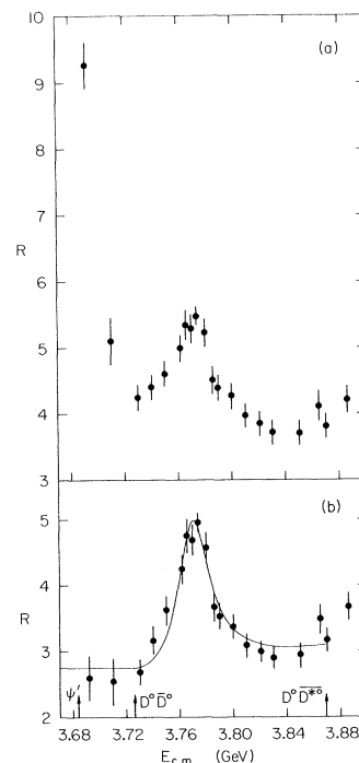
FIG. 2. R vs E_{c.m.} (a) before and (b) after corrections for radiative effects. The curve is a p -wave Breit-Wigner shape described in the text. The mass of the \psi' and the approximate positions of the thresholds for D^0\bar{D}^0 and D^0\bar{D}^{*0} production are indicated.
