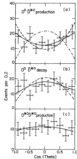
FIG. 1. (a) Production polar distribution of D^0 in Reaction (1). Solid curve corresponds to J_D^P = 0^+ and J_{D^*}^P = 1^+ . Dashed curve corresponds to J_D^P = 1^+ and J_{D^*}^P = 0^+ . Dash-dotted curve corresponds to spinless D and D^* ; here the argument "theta" is \Theta (see text). (b) Helicity polar distribution for D^0 in Reaction (1). Solid curve corresponds to J_D^P = 0^+ and J_{D^*}^P = 1^+ . Dashed curve corresponds to J_D^P = 1^+ and J_{D^*}^P = 0^+ ; here the argument "theta" is \theta . (c) Production polar distribution for D^0 in Reaction (2). Solid curve is deduced from fit; here the argument "theta" is \Theta .
