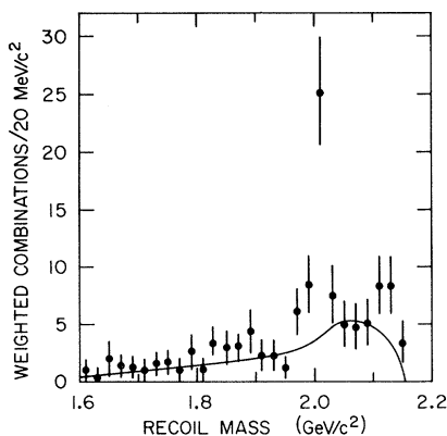
FIG. 2. Recoil mass spectra for the K^*\pi^+\pi^+ peak mass region, 1.86 to 1.90 \text{ GeV}/c^2 . The smooth curve is an estimate of the background obtained from the same region in the K^*\pi^+\pi^- spectrum.
