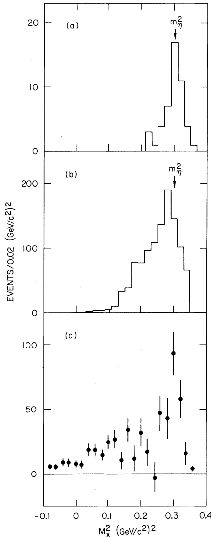
FIG. 3. Square of the recoil mass to the muon pair for (a) \psi' \rightarrow \psi \eta candidates with \eta \rightarrow charged modes; (b) \psi' \rightarrow \psi \pi^+ \pi^- events; (c) \psi' \rightarrow \psi + neutrals, with \psi' \rightarrow \psi \pi \pi subtracted.
