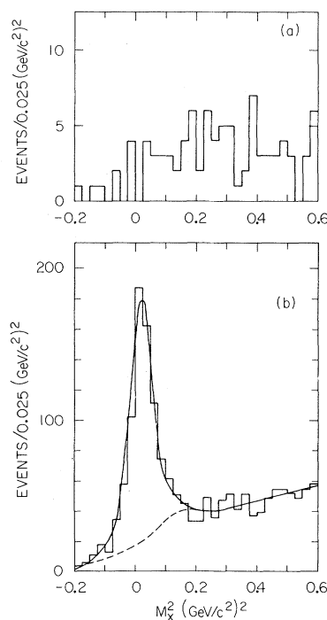
FIG. 2. Distribution of the four-prong events with a momentum imbalance greater than 200 MeV/c and a total charge zero at (a) c.m. energy of 3.0 GeV, (b) \psi(3095) ; the curve shows the Monte Carlo fit to the data.
