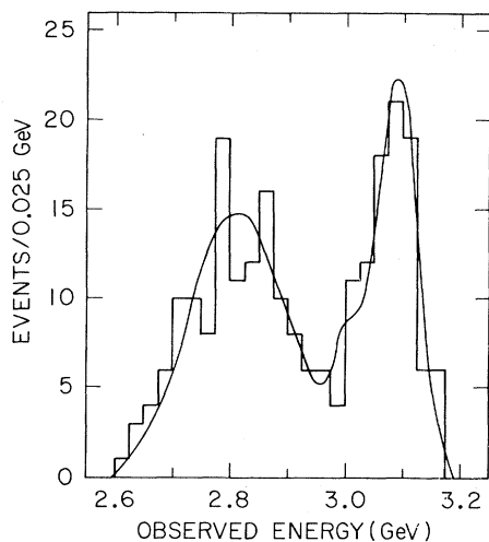
FIG. 1. Total energy of the charged tracks observed in four-prong events with a momentum imbalance of less than 0.100 GeV/c and a total charge equal to 0, assuming all particles are pions. The curve is a Monte Carlo fit to the data.
