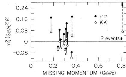
FIG. 4. Scatter plot of missing momentum versus square of the missing mass for two-prong events calculated for both the \pi\pi and KK hypothesis. Events with a dashed line (including both events which are off the right-hand side of the graph) contain evidence of two missing photons.
