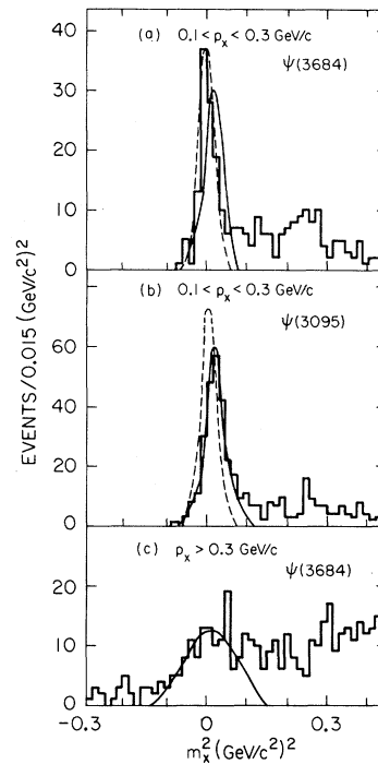
FIG. 2. The square of the missing mass for four-prong events. (a) \psi(3684) decays with 0.1 < p_x < 0.3 GeV/c. (b) \psi(3095) decays with 0.1 < p_x < 0.3 GeV/c. (c) \psi(3684) decays with p_x > 0.3 GeV/c. The solid and dashed lines give the predicted resolution functions for a missing \pi^0 and \gamma , respectively.
