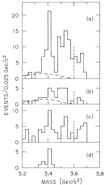
FIG. 3. Invariant-mass distributions after applying the constraint m_x^2=0 for the modes (a) 4\pi^\pm , (b) 6\pi^\pm , (c) \pi^+\pi^-K^+K^- , and (d) the sum of \pi^+\pi^- and K^+K^- . No missing-momentum cut has been made. Events above 3.60\text{-GeV}/c^2 in (a)–(c) are mainly events having no missing neutral and thus were fitted by the wrong hypothesis. The dashed line is the estimated background from (a) 4\pi^\pm\pi^0 and (b) 6\pi^\pm\pi^0 .
