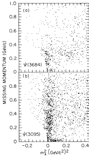
FIG. 1. Scatter plots of missing momentum versus square of the missing mass for four-prong events in (a) \psi(3684) decays and (b) \psi(3095) decays.
