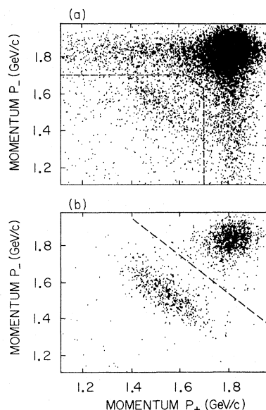
FIG. 1. Momentum of the negative lepton versus the momentum of the positive lepton for collinear (within 10^\circ ) two-prong events. e pairs (a) are separated from \mu pairs (b) using shower-counter pulse-height data. The cuts to select direct decays are marked by the dashed lines.
