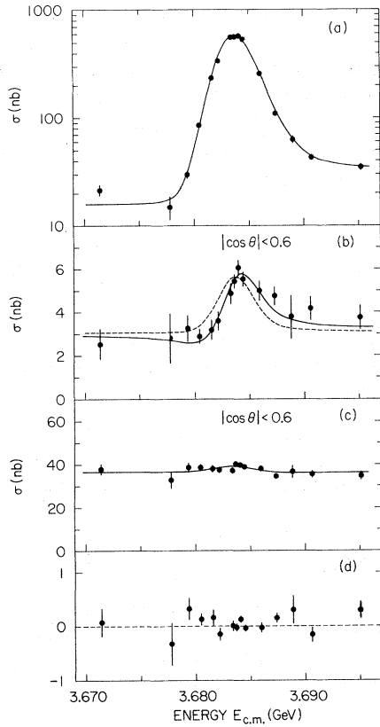
FIG. 2. Cross sections for (a) e^+e^- \rightarrow \text{hadrons} , (b) e^+e^- \rightarrow \mu^+\mu^- , and (c) e^+e^- \rightarrow e^+e^- versus center-of-mass energy. The solid curves represent the result of the fit to the data; the dashed line in (b) represents no interference. (d) The front-back asymmetry for the \mu^+ in e^+e^- \rightarrow \mu^+\mu^- .
