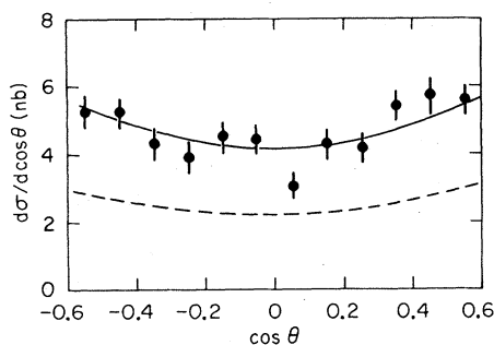
FIG. 3. Angular distribution of \mu^+ in e^+e^- \rightarrow \mu^+\mu^- in the center of the \psi(3684) peak. The solid curve is the fit assuming f(\theta) = 1 + \cos^2\theta ; the dashed curve is the QED contribution.
