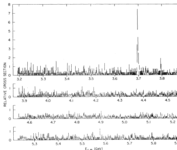
FIG. 1. Relative cross sections for e^+e^- \rightarrow hadrons.
